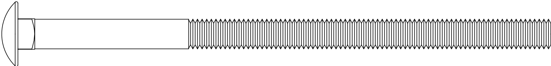
SBH-5 1/2" -13 x 9" Carriage Bolt ZP QTY; 1
